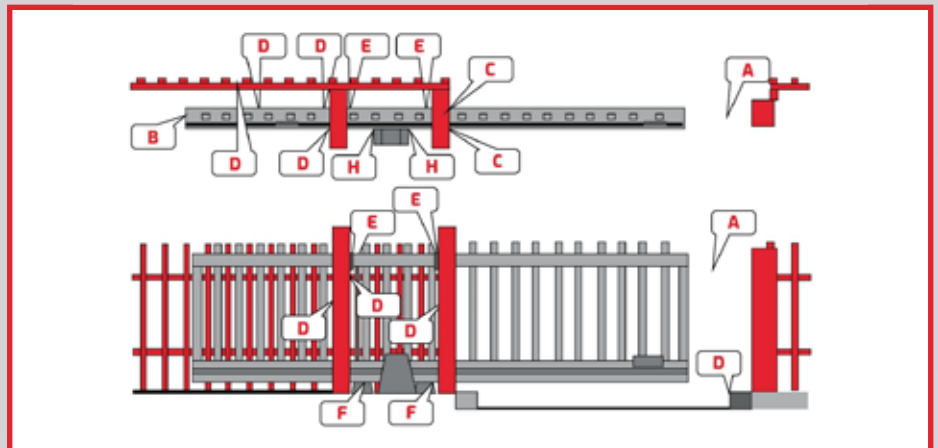
Figure 3.1 Elevation and plan view of an automatic cantilever sliding gate.
