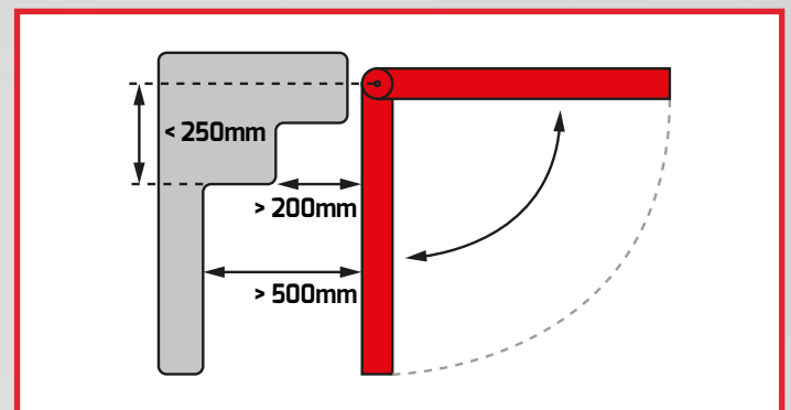
Figure 3.4 Gap reduction to reduce crushing hazard.
